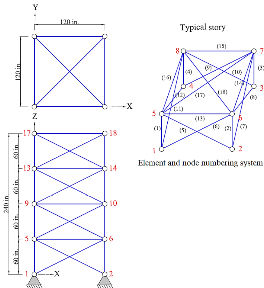
Figure 4. 72-bar truss
